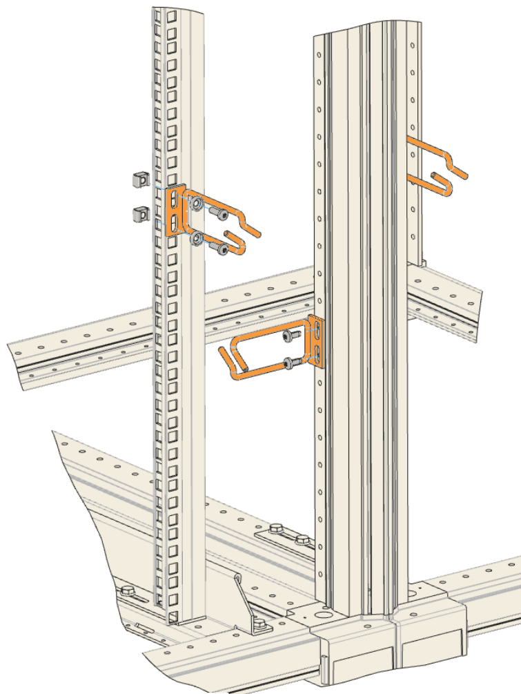
viewVue de face — Front view
