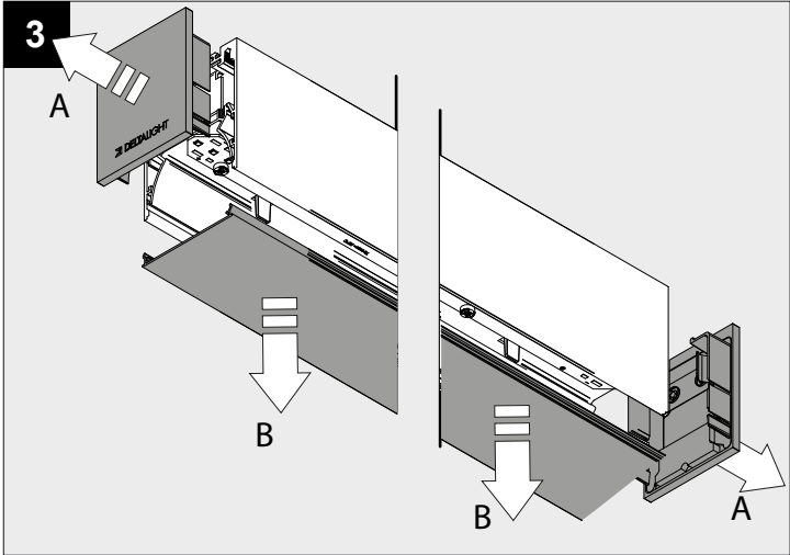
SURFACE MOUNTING
