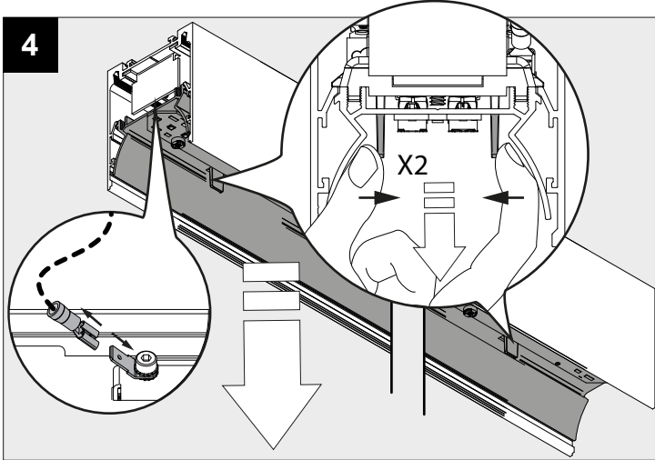
SUSPENDED MOUNTING
