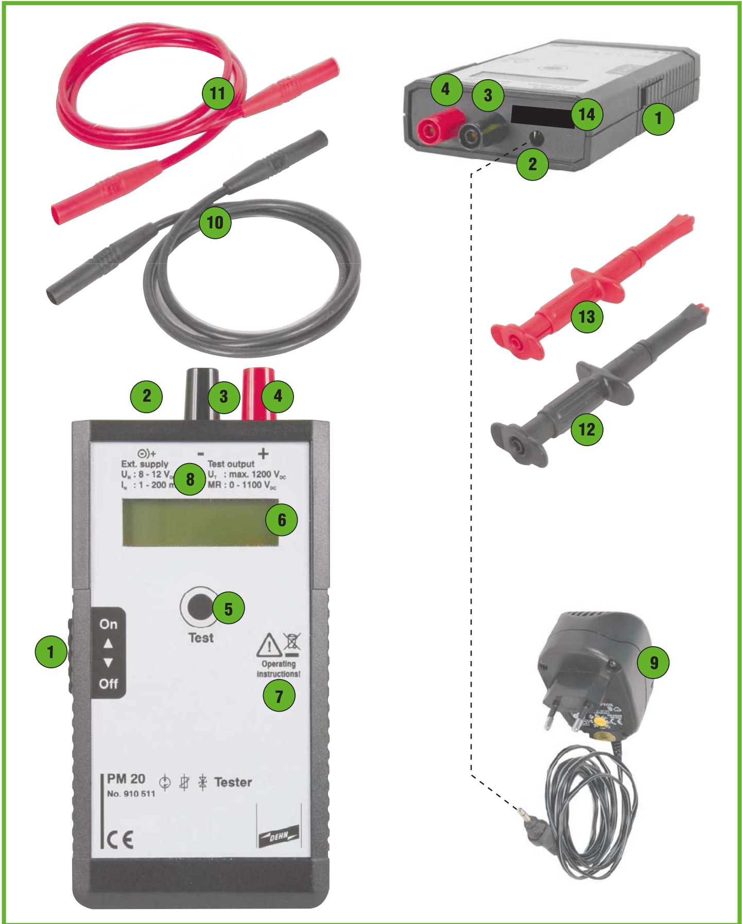
Figure 2 Device features
