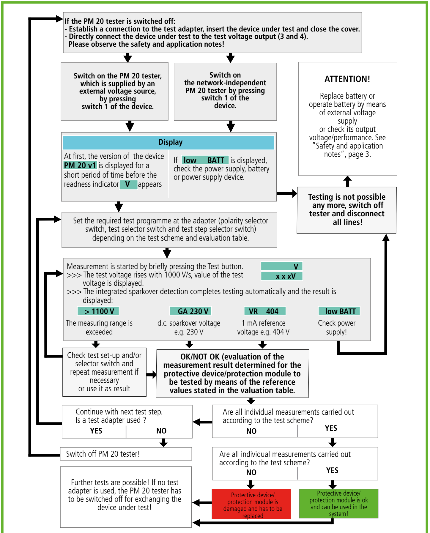
Figure 6 Test procedure
