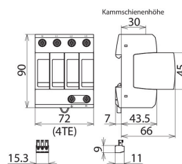
Dimensions DG M TT 5 CI 275 NL FM
