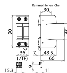
Dimensions DG M TN 275 NL FM
