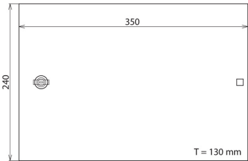
Dimensions DPG LSA 60 P
