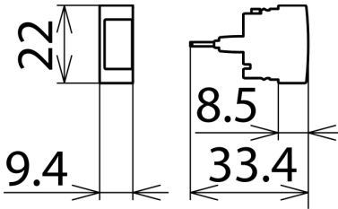
Dimensions DRL RE 12
