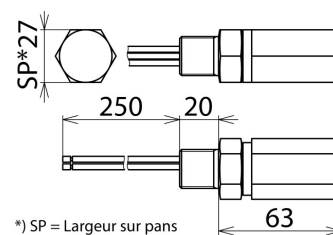
Dimensions DPI CD EXI+D 2X24 N
