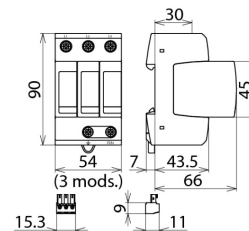
Dimensions DG M TNC 275 FM
