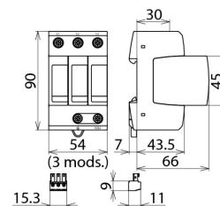
Dimensions DG M TNC 440 FM
