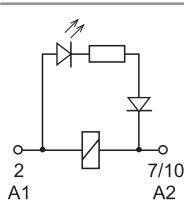
C: Variantes 3, 5, 54 LED (AC)
