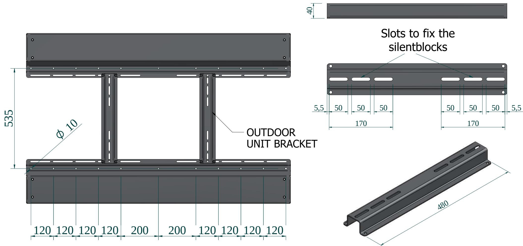
OUTDOOR UNIT BRACKET (Detail)
