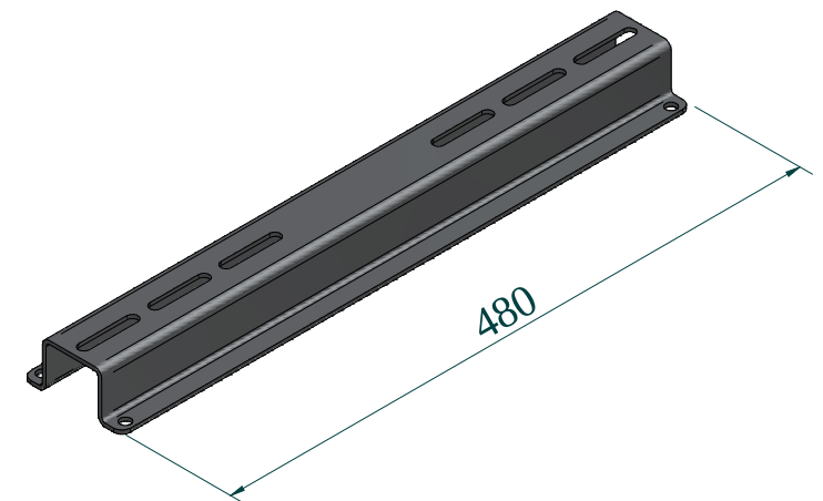
OUTDOOR UNIT BRACKET (Detail)
