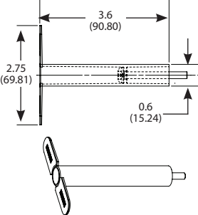
PZBR3.5 3.5" Bend Radius Post Kit
