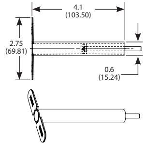
PZBR4 4" Bend Radius Post Kit
