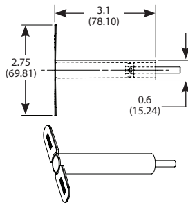
PZBR3 3" Bend Radius Post Kit
