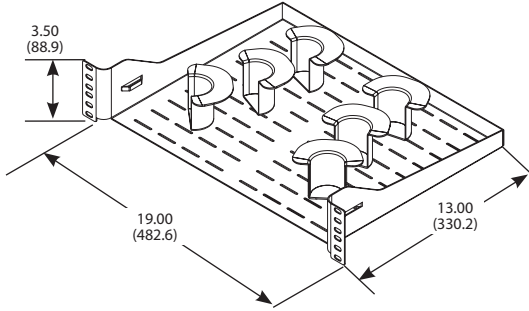
PZCHSM2 Horizontal Slack Manager, 2 RU includes (2) PZBR4 Kits
