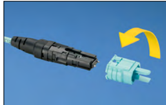
Remove Outer Housing, Flip and Reinstall
