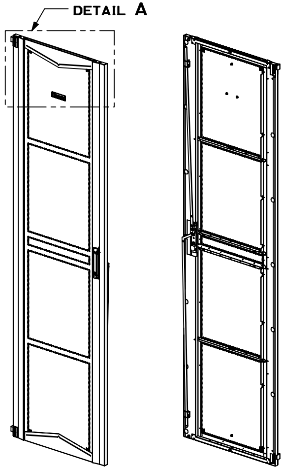
ISO VIEW - FRONT ISO VIEW - REAR
