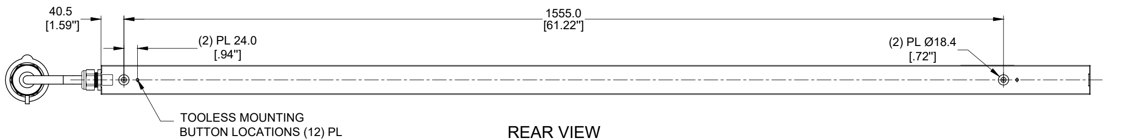
REAR VIEW
