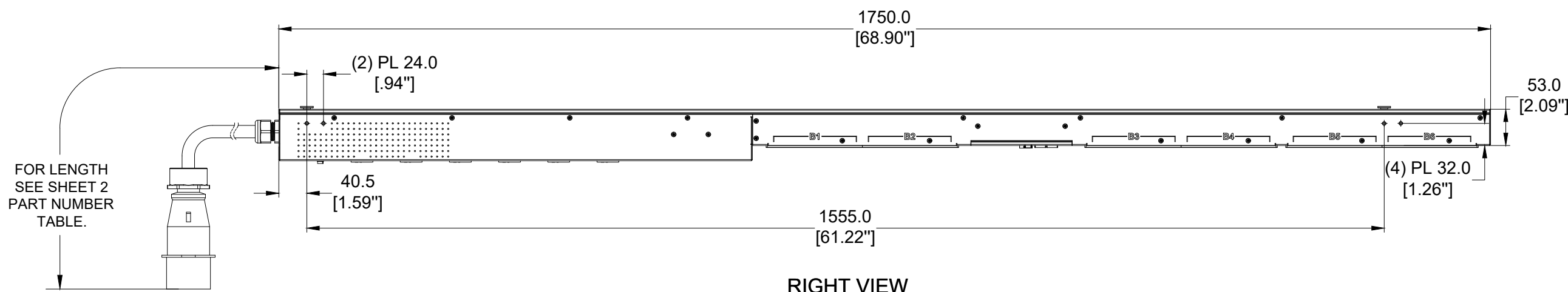
RIGHT VIEW
