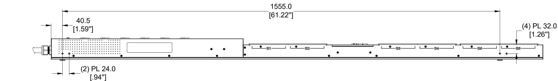
LEFT VIEW
