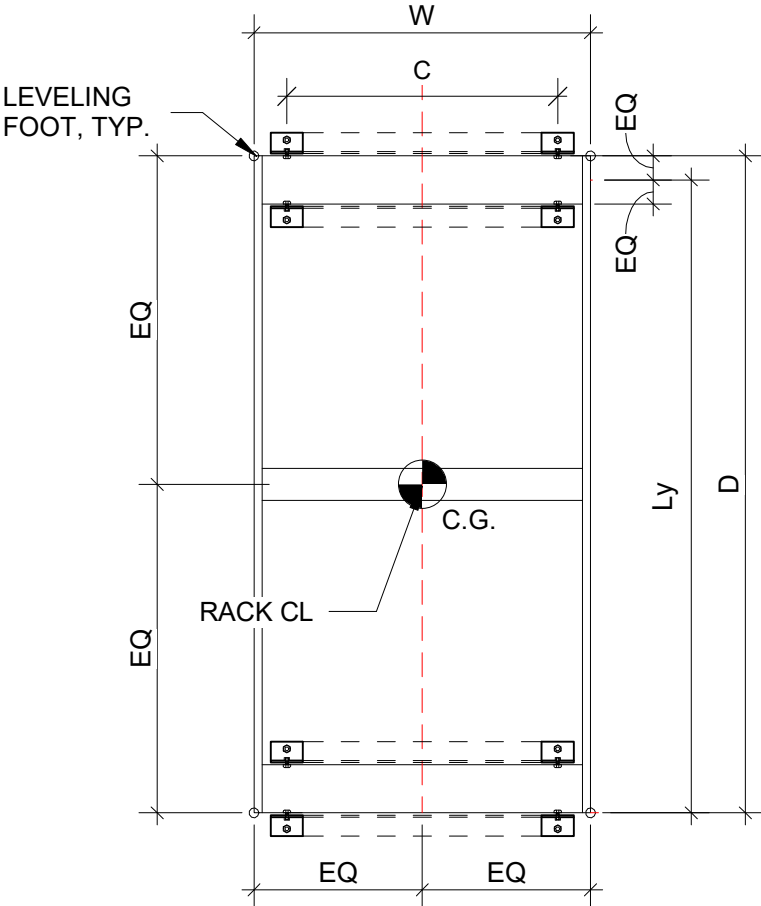
CABINET BASE FRAME PLAN
