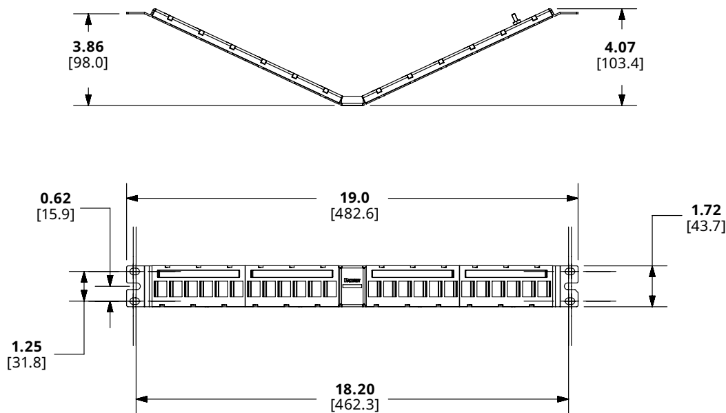
Shielded Keystone 24-Port Angeled Patch Panel — SKPPA24BL
