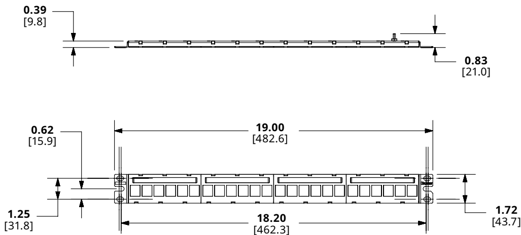
Shielded Keystone 24-Port Patch Panel — SKPP24BL
