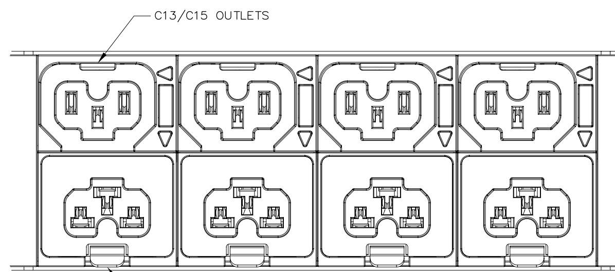
DETAIL A SCALE 1:1
