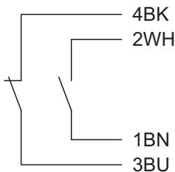
Câble 1NF + 1NO
