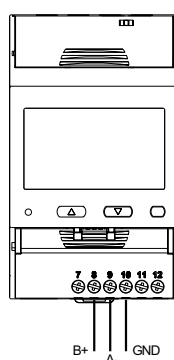
Fig. 15 Port RS485
