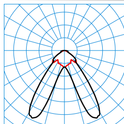
E-Line M-DA LED4000-840 IP54 TX053289
