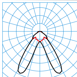
E-Line M-DA LED4000-830 IP54 TX053286
