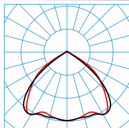
E-Line M-B LED6500-840 IP54 TX053275
