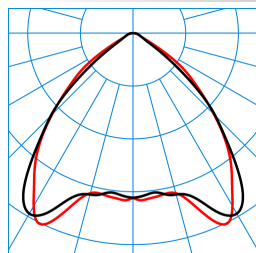
E-Line M-TB LED6500-830 IP54 TX053396
