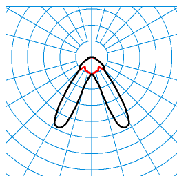
E-Line M-DA LED6500-840 IP54 TX371149
