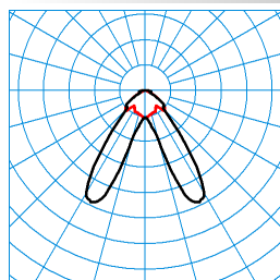
E-Line M-DA LED6500-840 TX371550
