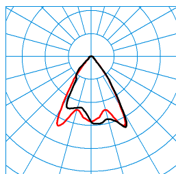
InperiaLP C05 WW-MR 1800-830 01 + ZN-PC TX045528 ■ C0 - C180 ■ C90 - C270 DIN 5040: A60 UTE: 1,00 A CEN Flux Code: 84 94 98 99 100 30 50 60 1
