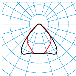
C-Line B LED6000-840 TX373821
