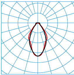
C-Line T LED4000-830 TX046742
