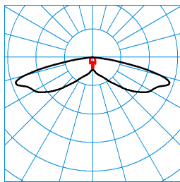
Publisca P1-SB3L/1200-740 2G1S ETDD (CLO initial value) TX300291 ■ C0 - C180 ■ C90 - C270 DIN 5040: A30 UTE: 1,00 l CEN Flux Code: 31 65 93 100 100
