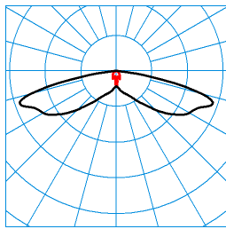
Publisca P1-SB3L/1200-740 2G1S ETDD (CLO end value) TX300968 ■ C0 - C180 ■ C90 - C270 DIN 5040: A30 UTE: 1,00 l CEN Flux Code: 31 65 93 100 100
