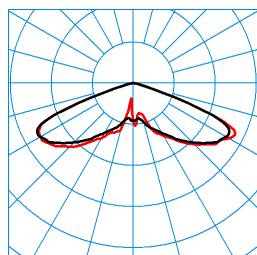
Publisca P1-RB6L/2600-740 3G1S ETDD (CLO initial value) TX301880 DIN 5040: A20 UTE: 1,00 J CEN Flux Code: 20 57 98 100 100
