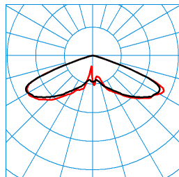
Publisca P1-RB6L/2600-740 3G1S TX047598 DIN 5040: A20 UTE: 1,00 J CEN Flux Code: 20 57 98 100 100
