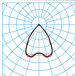
E-Line M-B19 LED5000-830 TX050724
