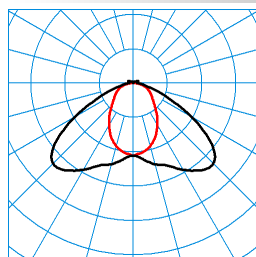
C-Line XB LED6000-830 03 TX374145
