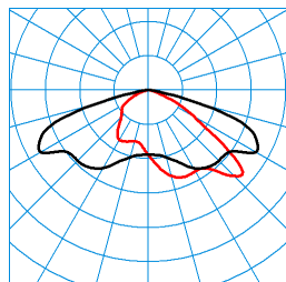
Jovie 70-AB7L-LRA/24000-730 24G1 ET (CLO initial value) TX301063 ■ C0 - C180 ■ C90 - C270 DIN 5040: A30 UTE: 1,00 G CEN Flux Code: 35 73 97 100 100
