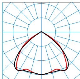
7651 LightP B-B-B 65-830ETDD L75 03 (225) TX557008
