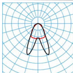
ELINE HE+ LDAN80 840 L225 1 20
