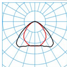
ELINE FL LVW60 865 L225 1 20
