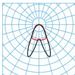
ELINE HE LDAN60 840 L150 4 20 ■ C0 - C180
