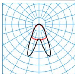
ELINE HE LDAN60 827 L150 2 20 ■ C0 - C180
