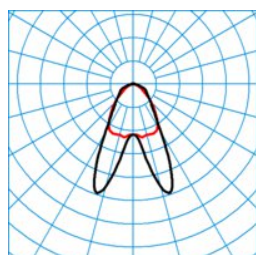
ELINE HE LDAN60 865 L150 3 20 ■ C0 - C180
