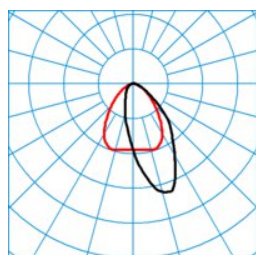
ELINE HE LAN100 840 L225 4 20 ■ C0 - C180 DIN 5040 3 = A50 UGR I 3 = 0,0 UGR q 3 = 0,0 UTE 3 = 0.98 C + 0.02 T CEN flux code = 63 89 98 98 100 0 6 44 2
