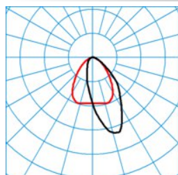
ELINE HE LAN100 827 L225 2 20 ■ C0 - C180 DIN 5040 = A50 UTE = 0.98 C + 0.02 T CEN flux code = 63 89 98 98 100 0 6 44 2
