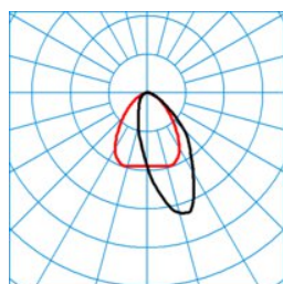
ELINE HE LAN100 865 L225 3 20 ■ C0 - C180 DIN 5040 2 = A50 UGR I 2 = 0,0 UGR q 2 = 0,0 UTE 2 = 0.98 C + 0.02 T CEN flux code = 63 89 98 98 100 0 6 44 2
