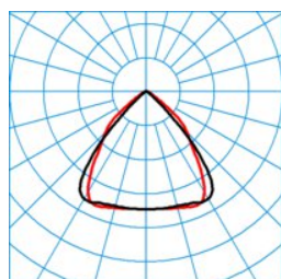
ELINE FL HE LW1940 840 L150 4 20
