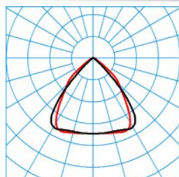
ELINE FL HE LW1940 827 L150 2 20
