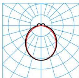
ELINE FL HE DSL100 840 L225 4 20
