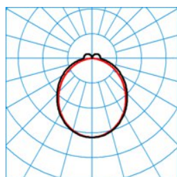
ELINE FL HE DSL100 865 L225 3 20
