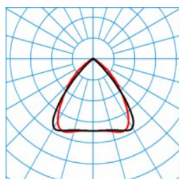
ELINE FL HE LN100 865 L225 3 20
