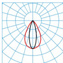
ELINE HE LEN60 840 L225 4 50
