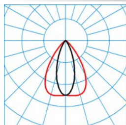
ELINE HE LVN40 840 L150 1 50
