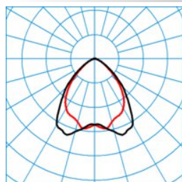
ELINE LW100 840 L225 1 50
