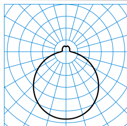
74R G2 WD2 DW 42-840 ET IP44 TX784165
