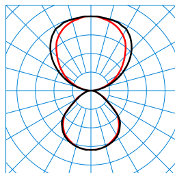
Luceos D/H2-L CDP 8400-840 ETDD 03 (Pendant ZS/ZST) TX547699
