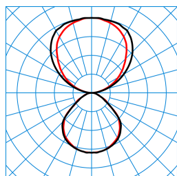
Luceos D/H2-L CDP 8400-830 ETDD 01 (Pendant ZS/ZST+EB3) TX547705
