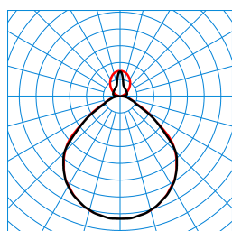
Luceos D/H2-L CDP 8400-830 ETDD 01 (Ceiling D2 ZD/03+EB3) TX547718
