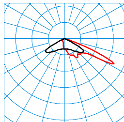
LnPlus 60-AM19L-SLR2/26000-727 24G1 ET (CLO initial value) TX390185 DIN 5040: A30 UTE: 1,00 J CEN Flux Code: 28 76 99 100 100 ■ C0 - C180 ■ C90 - C270
